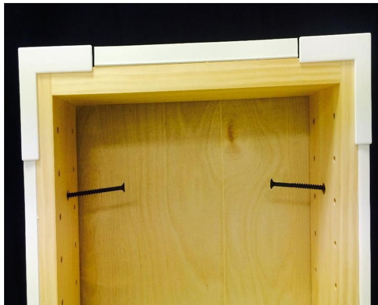
Image 3 screwing the cabinet to studs in wall
